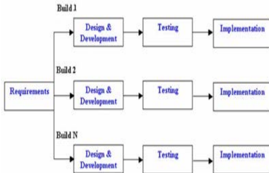
Gambar 1 : Siklus Model Incremental [Deden, 2011]
